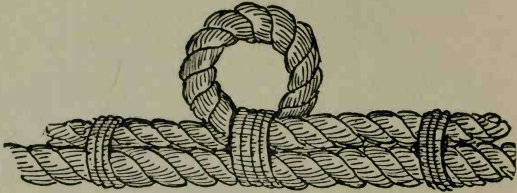
FIG. 96.—Lashed cut-splice.
